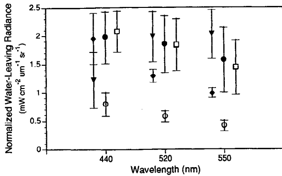
Figure 2. Mean ( \pm\sigma ) normalized water-leaving radiances ( nLw ) for coccolithophorid blooms (solid circles), "clear" blue water (open circles), haze (solid triangles), sediments (solid diamonds), and whittings (open squares) at CZCS band wavelengths.
